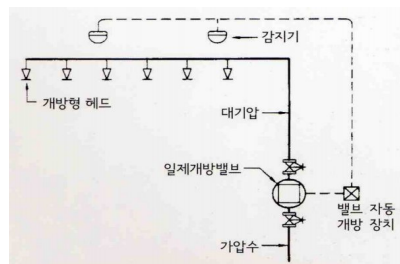
일제살수식(Deluge system)
