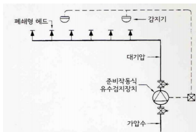
준비작동식(Preaction system)
