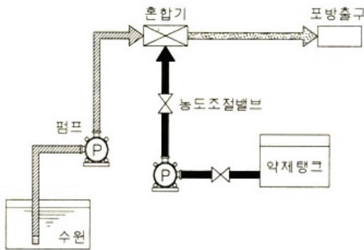
Pressure side proportioner type
